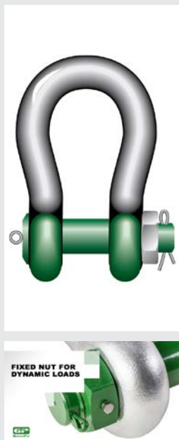
Green Pin Fixed Nut Heavy Duty Polar Shackle Grade 8
